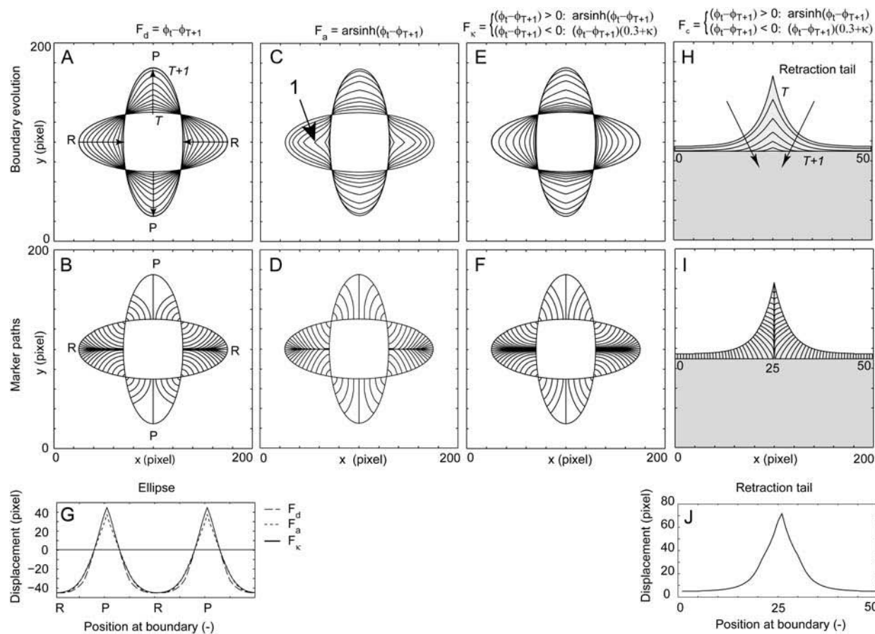
FIGURE 6 Evaluation of the LSM on two test cases using three different speed functions. The computational grid size was (3,3) pixels and the adaptable time step of the integrator was on average 0.1. See text for a discussion of the difference in speed functions.
